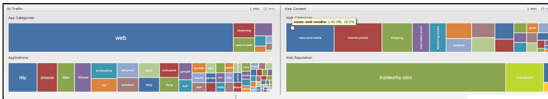
Figure 59 AppRF Dashboard
