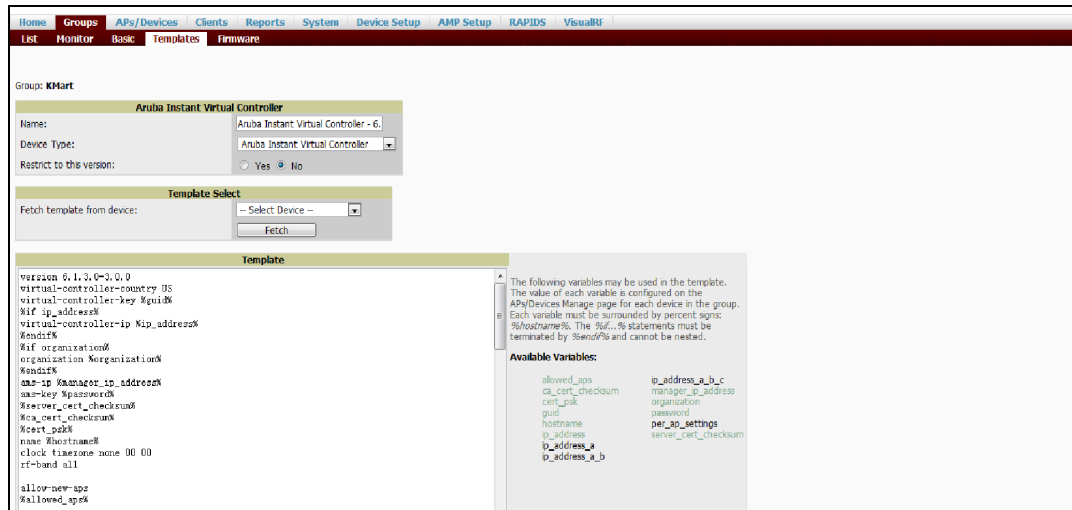
Figure 83 Template-based Configuration
