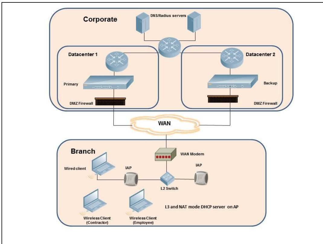
Figure 123 Scenario 3—IPSec: Multiple Datacenter Deployment with Primary and Backup Switches for Redundancy
