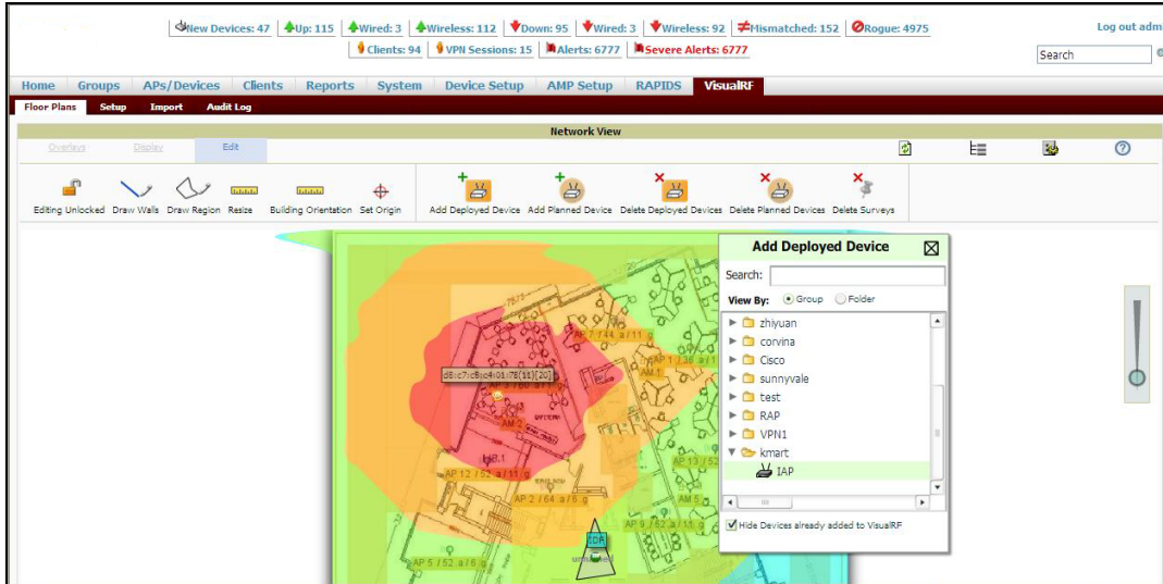
Figure 84 Adding an OAW-IAP in VisualRF
